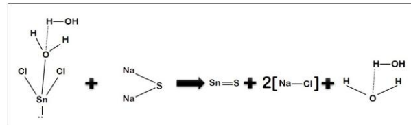
Fig. 2 Chemical equation of formation of SnS nanoparticles
